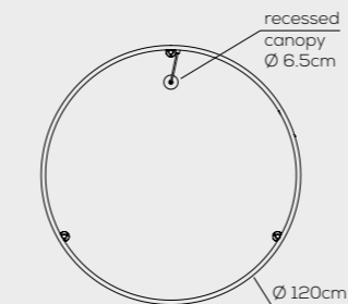
rosone incasso / recessed canopy
