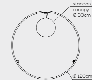
rosone standard / standard canopy
